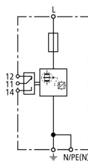
Basic circuit diagram DBM 1 CI 440 FM
