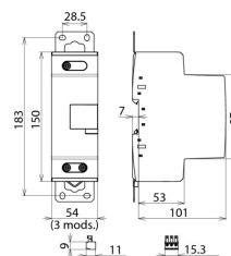
Dimension drawing DBM 1 CI 440 FM
