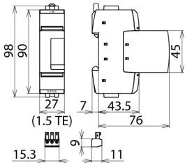
Dimension drawing DG SE H 1000 VA FM
