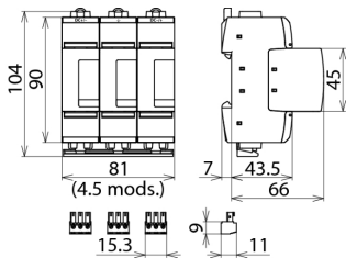
Dimension drawing DG ME YPV SCI1500 FM
