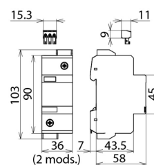
Dimension drawing DG 1000 FM
