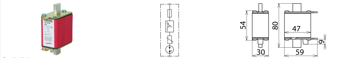
Basic circuit diagram VA NH00 280 Dimension drawing VA NH00 280 Surge arrester with a varistor and a spark gap connected in series; for use in NH00 fuse holders for TT and TN systems, optionally available with special indicator for remote signalling.
