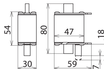
Dimension drawing VA NH00 280 FM
