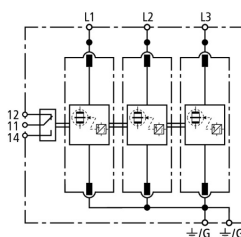
Basic circuit diagram DB MU 3PY 480 3W+G R
