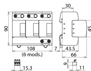
Dimension drawing DB MU 3PY 480 3W+G R
