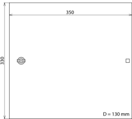
Dimension drawing DPG LSA 120 P
