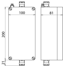
Dimension drawing ALGA 5
