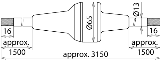
Dimension drawing EXFS KU
