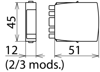
Dimension drawing BXT ML2 BD S 15
