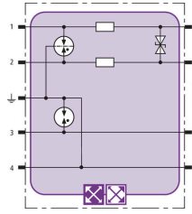
Basic circuit diagram BXT ML2 BD S 15
