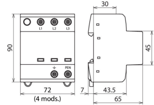
Dimension drawing DSH TNC 255
