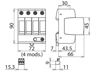
Dimension drawing DG MU 3PY 208 4W+G R
