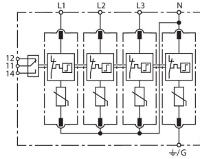
Basic circuit diagram DG MU 3PY 208 4W+G R
