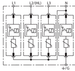
Basic circuit diagram DG MU 3PH 240 4W+G
