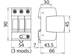
Dimension drawing DG MU SPN 240 3W+G
