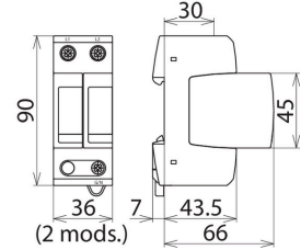
Dimension drawing DG MU CGD 480 3W+G
