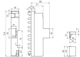
Dimension drawing DSH ZP 2 TNS 255
