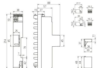
Dimension drawing DSH ZP 2 SG TNS 255
