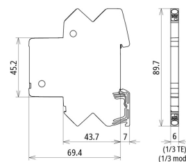
Dimension drawing BCO CL2 E 24
