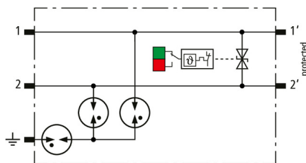
Basic circuit diagram BCO ML2 BD HC5A 24
