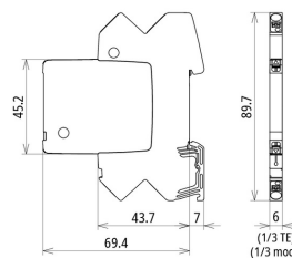
Dimension drawing BCO ML2 BD EX 24
