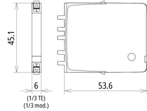
Dimension drawing BCO MOD ML2 B 180
