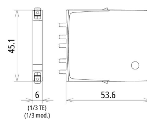
Dimension drawing BCO MOD ML2 BD HC5 A 24
