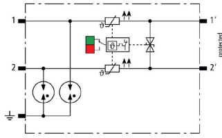
Basic circuit diagram BCO MOD ML2 BPD 24
