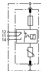
Basic circuit diagram DG MOD E CI 440
