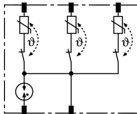
Basic circuit diagram DR MOD 4P 255
