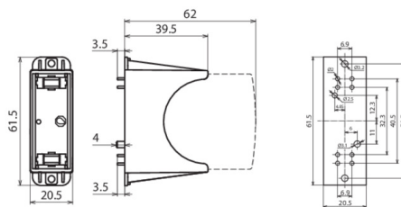
Dimension drawing DG PCB NPE
