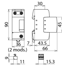
Dimension drawing DGPH M 255
