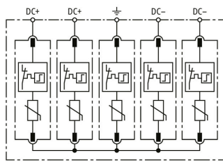
Basic circuit diagram DCU 2 YPV 1+2 1000 2M 2S FM
