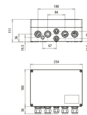
Dimension drawing DCU 2 YPV 1+2 1000 2M 2S FM
