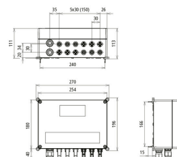
Dimension drawing DCU 2 YPV 1100 3M 1S MC4 FM
