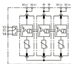
Basic circuit diagram DCU 2 YPV 1100 3M 1S MC4 FM
