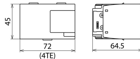
Dimension drawing DV MOD TNS 255
