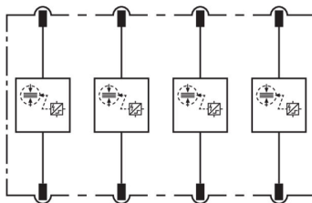
Basic circuit diagram DV MOD TNS 255
