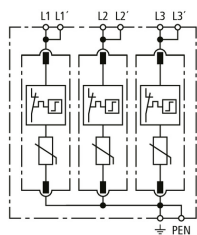
Basic circuit diagram DG MP TNC 275 FM
