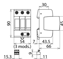
Dimension drawing DG MP TNC 275 FM
