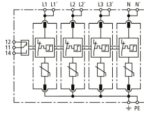
Basic circuit diagram DG MP TNS 150 FM
