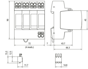
Dimension drawing DG MP TNS 150 FM
