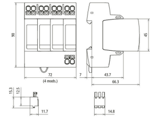
Dimension drawing DG MP TNS 385 FM
