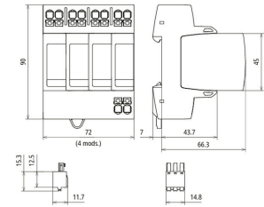
Dimension drawing DG MP TT 275 FM
