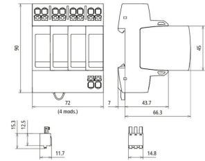
Dimension drawing DG MP TT 320 FM
