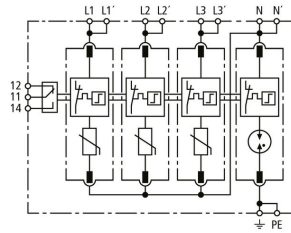
Basic circuit diagram DG MP TT 320 FM
