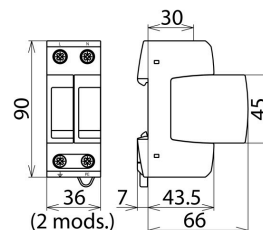
Dimension drawing DG MP TN 275 FM
