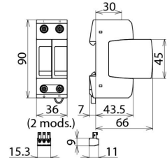
Dimension drawing DG MP TT 2P 275 FM
