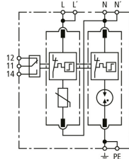
Basic circuit diagram DG MP TT 2P 320 FM
