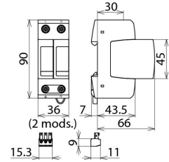
Dimension drawing DG MP TT 2P 320 FM
