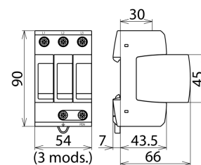
Dimension drawing DG M TNC 440
