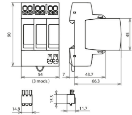
Dimension drawing DG MP YPV 1500 FM
