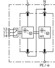
Basic circuit diagram DV M2 TT 2P 255 FM
