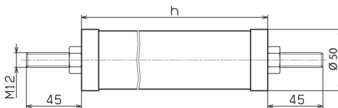
Dimension drawing DMi 6 10 1 L
