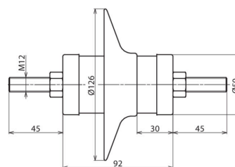
Dimension drawing DMI 3 10 1 N
