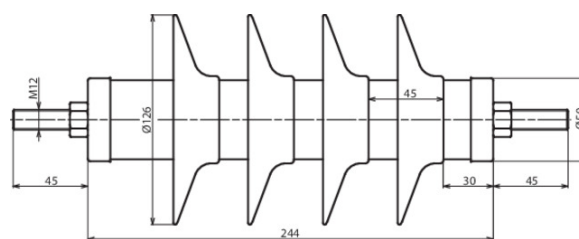
Dimension drawing DMI 27 10 1 N
