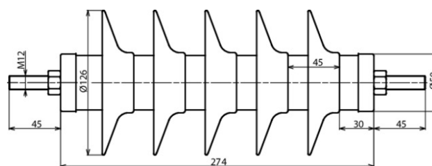
Dimension drawing DMI 31 10 1 N
