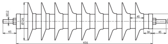
Dimension drawing DMI 51 10 1 N
