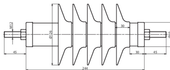
Dimension drawing DMI 27 10 1 H
