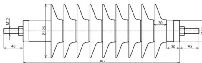
Dimension drawing DMI 36 10 1 H
