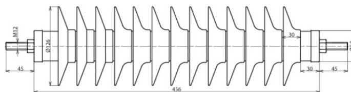
Dimension drawing DMI 51 10 1 H
